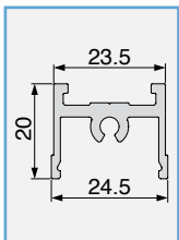
Frame profile.
