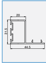
Edge profile / photocell holder.
