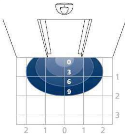
Detection range based on sensitivity adjustment
