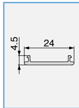
Latch profile.
